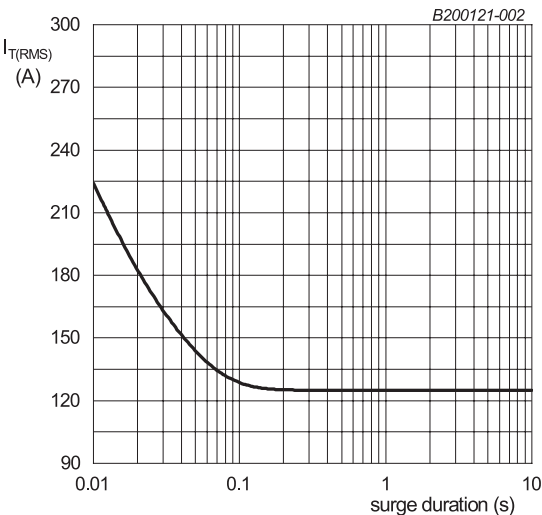
f = 50\text{ Hz} ; T_{mb} = 118\text{ }^{\circ}\text{C} Fig. 2. RMS on-state current as a function of surge duration; maximum values
