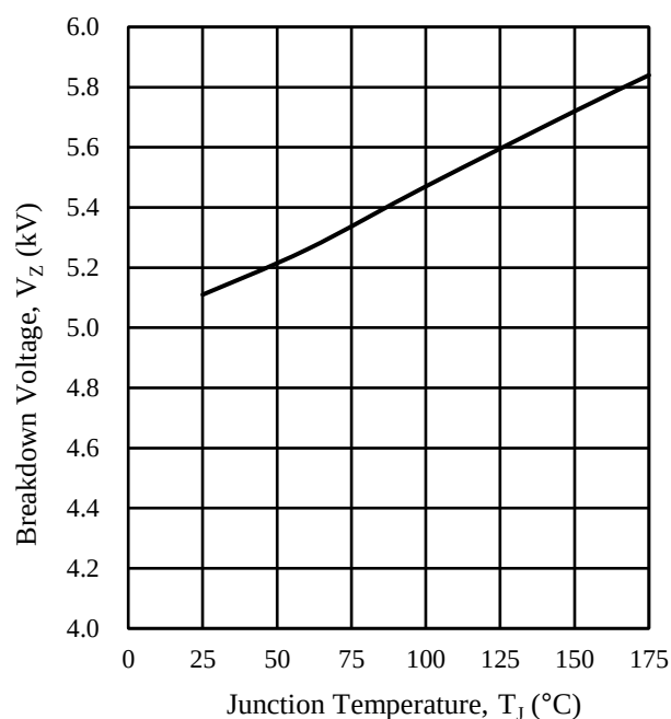
Figure 13. V_Z vs. T_J ( I_Z = 100 μA)
