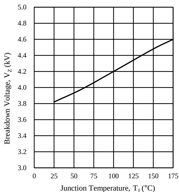
Figure 9. V_Z vs. T_J ( I_Z = 100 μA)
