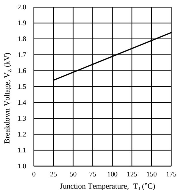
Figure 5. V_Z vs. T_J ( I_Z = 100 μA)
