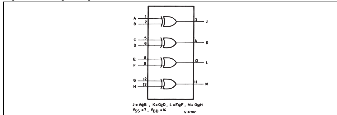
Figure 3. Logic diagram
