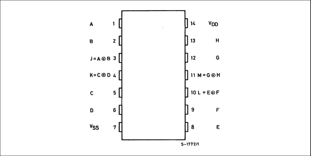
Figure 1. Pin connections
