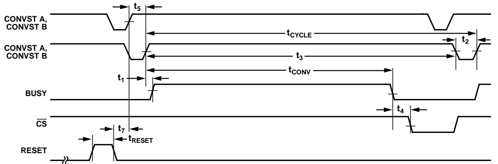
Figure 2. CONVST Timing—Reading After a Conversion
