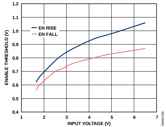
Figure 26. Typical EN Thresholds vs. Input Voltage ( V_{IN} )
