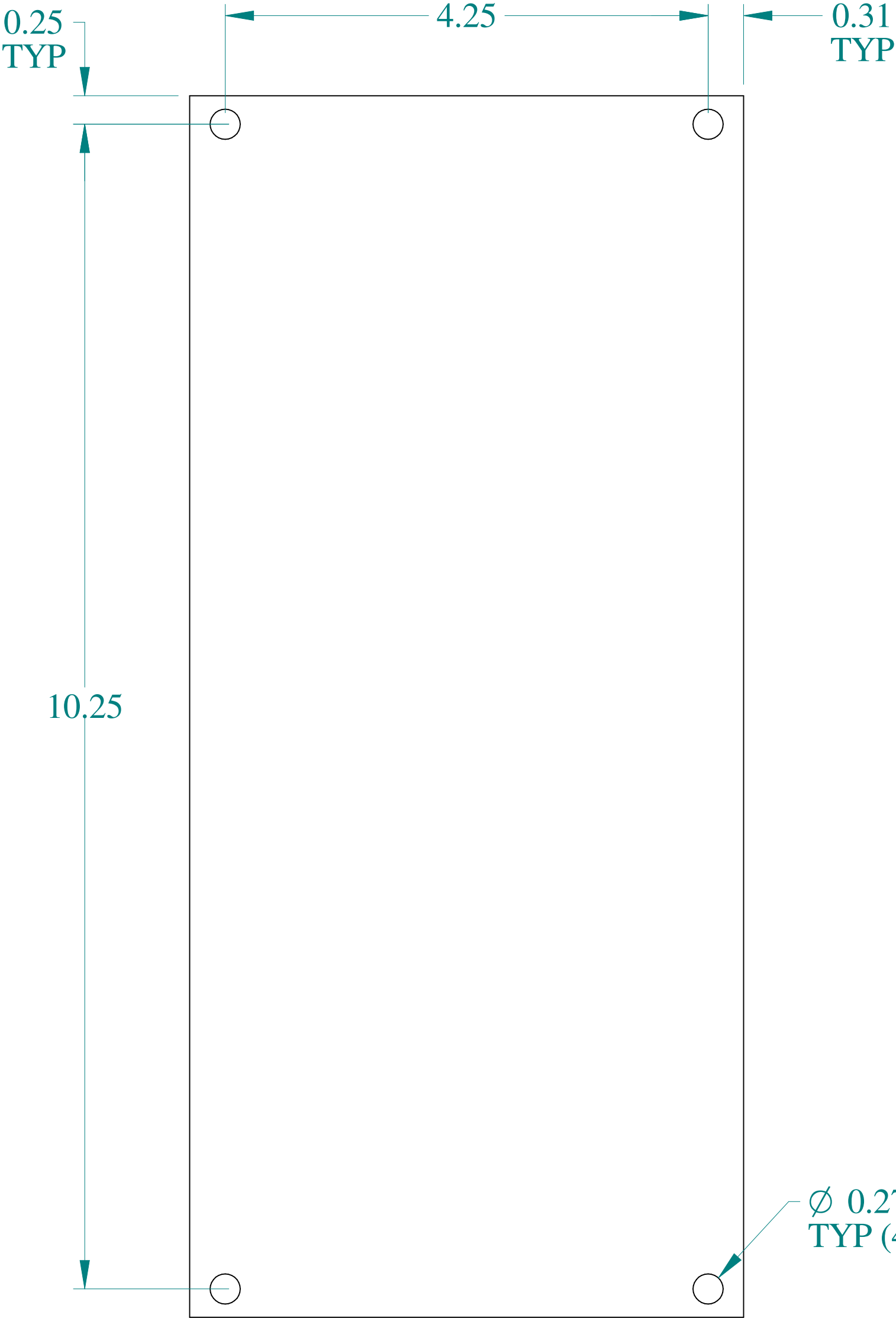
FRONT VIEW
