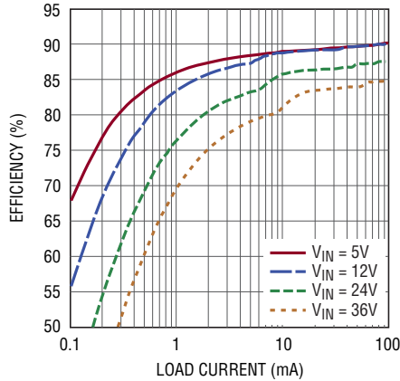
Burst Mode Efficiency, V OUT = 12V, L = 15μH
