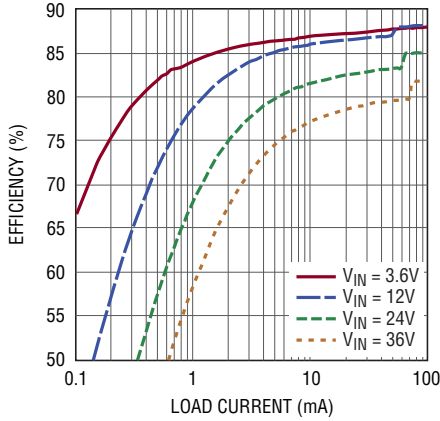
Burst Mode Efficiency, V OUT = 5V, L = 15μH, Non-Bootstrapped
