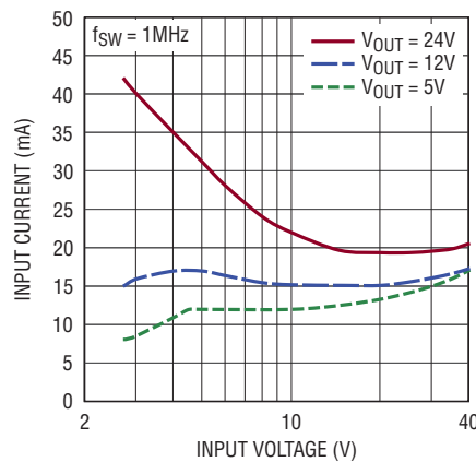
PWM Mode No-Load Input Current vs V IN
