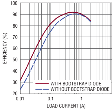
Efficiency vs Load Current VIN = 12V
