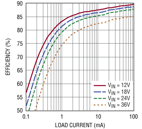
Burst Mode Efficiency, V OUT = 24V, L = 15μH
