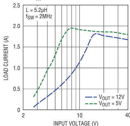
Maximum Load Current vs V IN , PWM Mode
