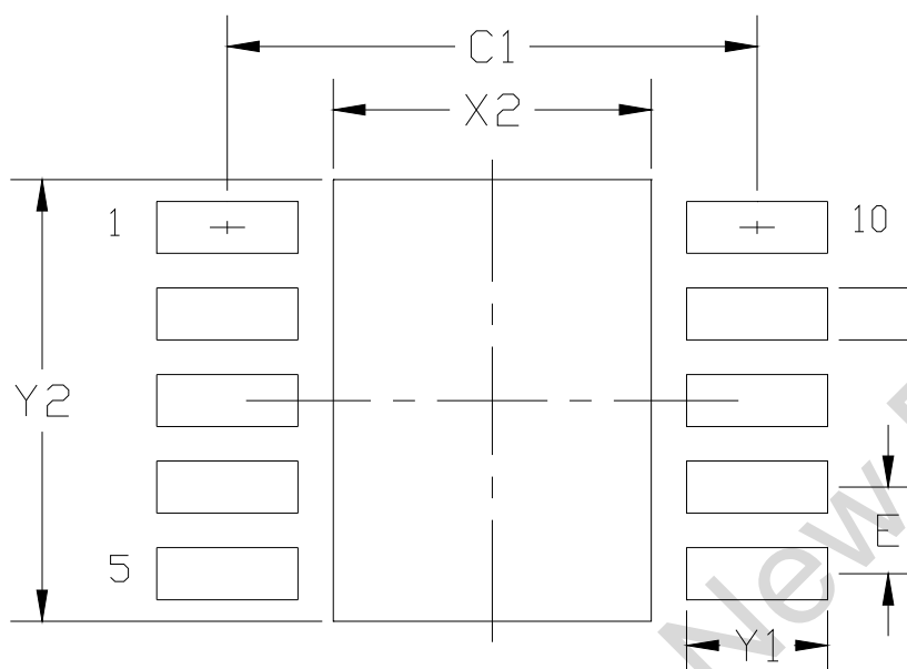
Figure 3.3. DFN-10 Landing Diagram
