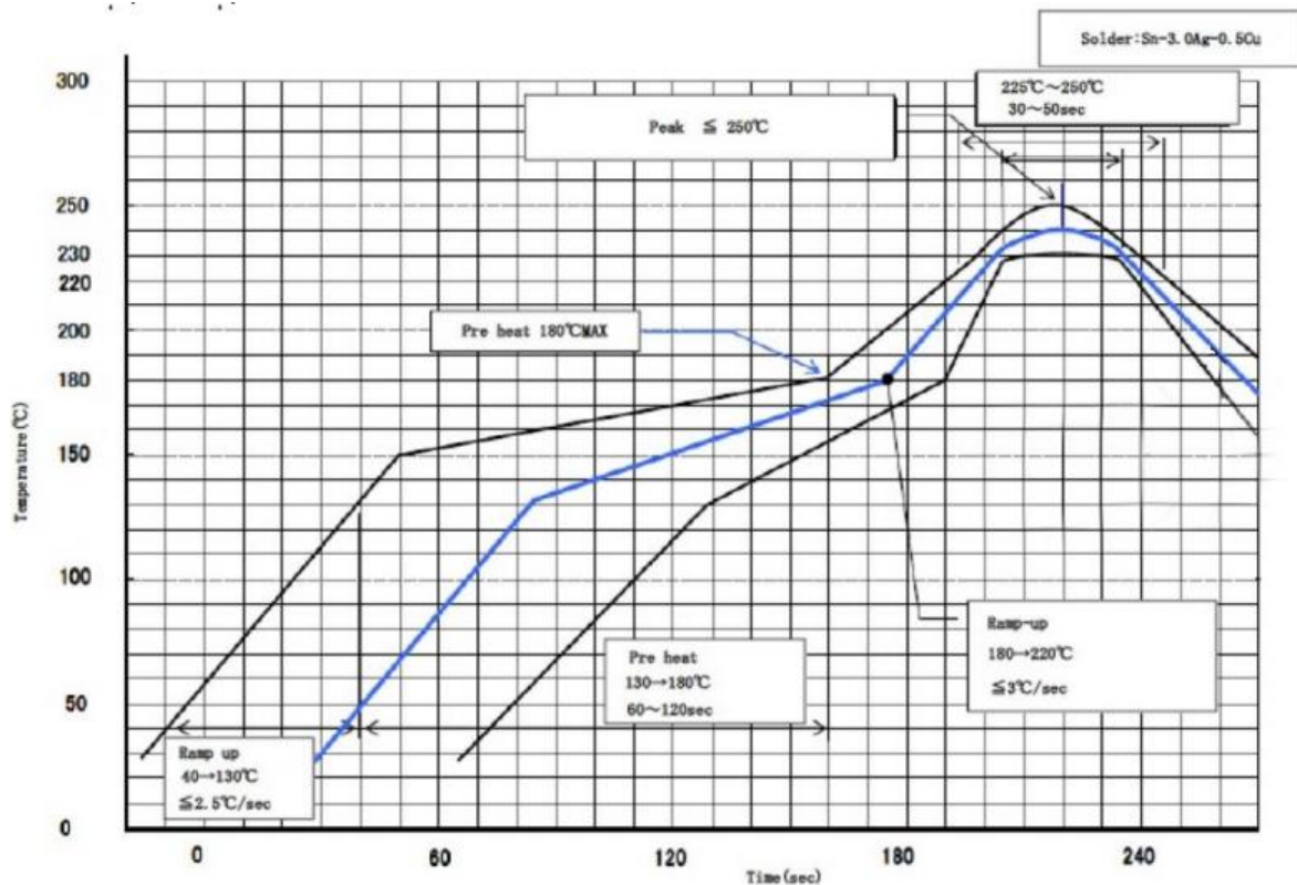
Figure 9: Recommend reflow profile
