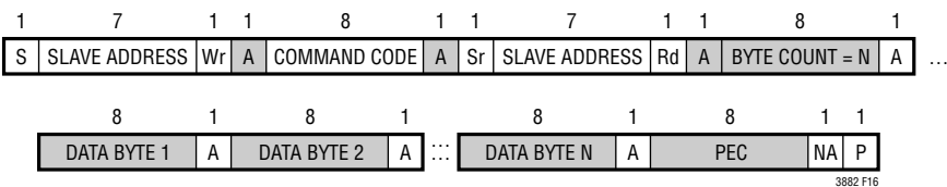
Figure 16. Block Read Protocol with PEC
