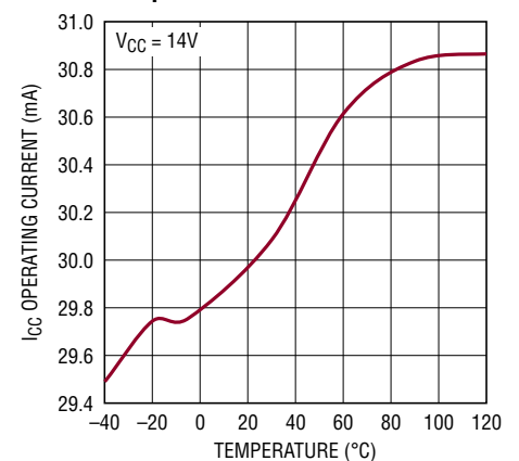
IC Operating Current vs Temperature
