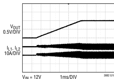
Soft-Start Ramp
