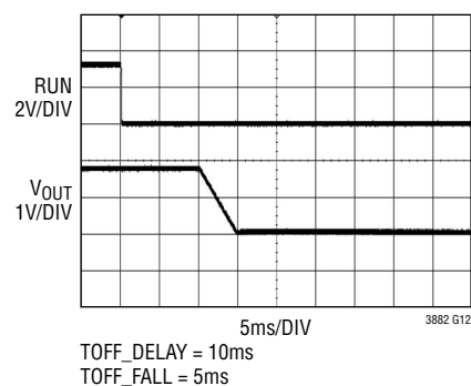
Soft-Off Ramp
