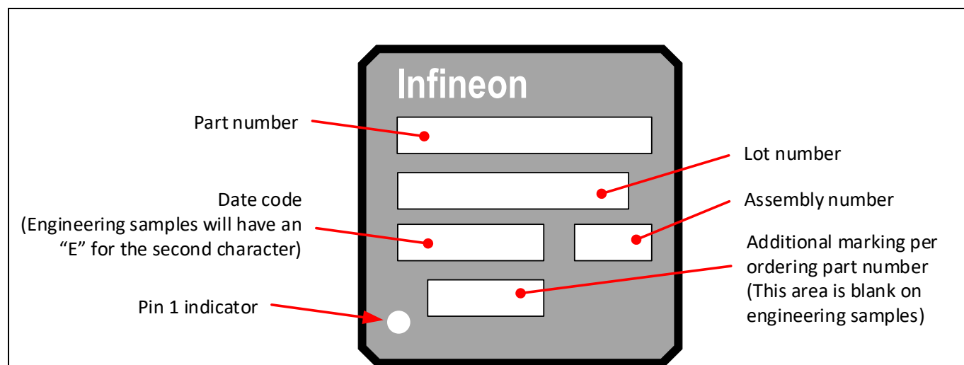
Figure 2 Package marking
