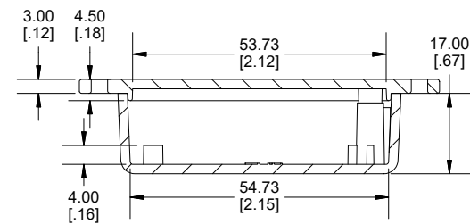
SIDE VIEW SECTION B-B
