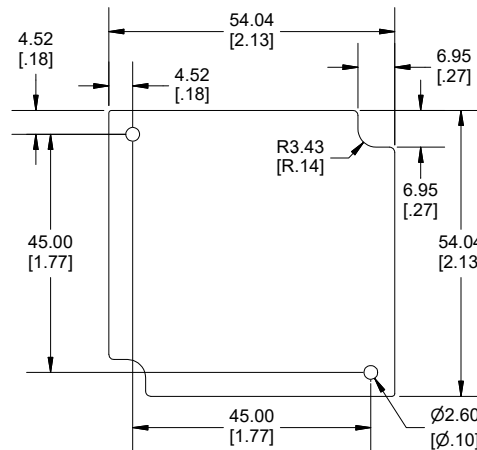
MAXIMUM P.C. BOARD SIZE
