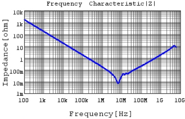
GJ821BR71H105KA12 |Z| DCOV, 25degC
