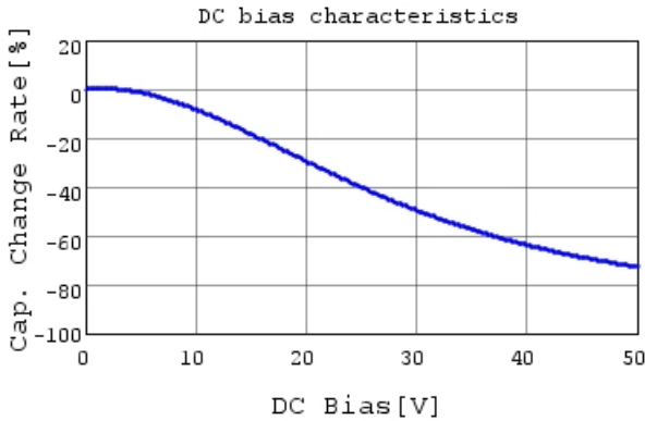
GJ821BR71H105KA12 C-DC bias capchange, 25.0c
