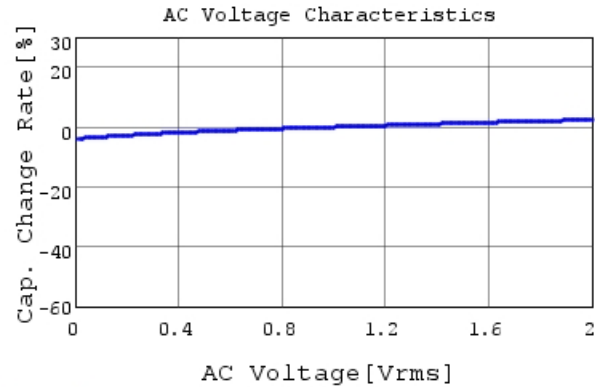
GJ821BR71H105KA12 C-AC Voltage capchange, Dc
