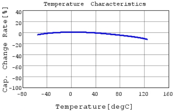
GJ821BR71H105KA12 C-Temp. capchange, DC0.0V,
