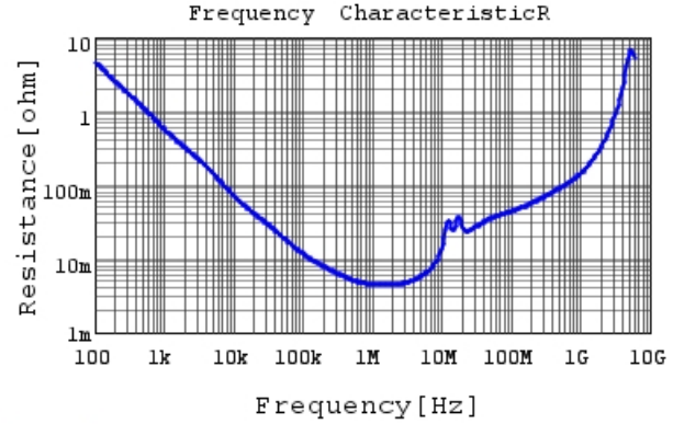
GJ821BR71H105KA12 R DCOV, 25degC
