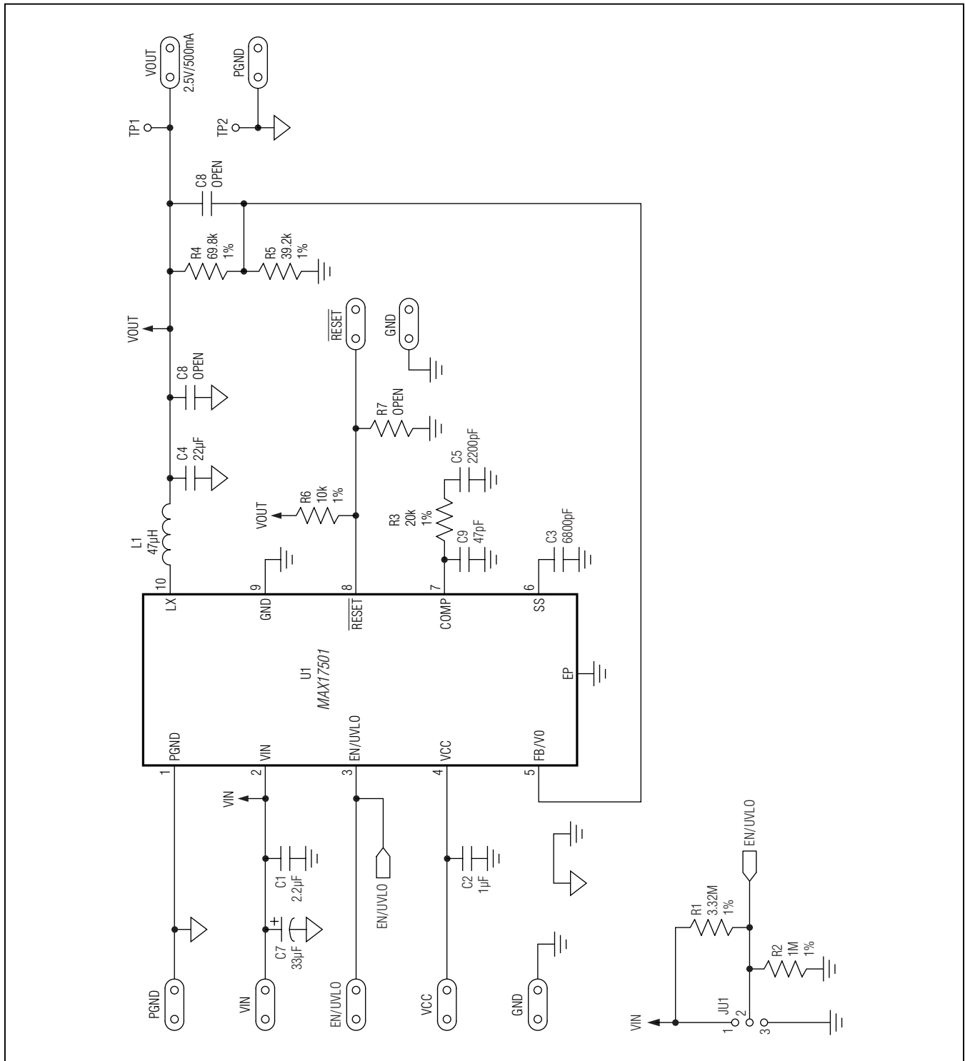
Figure 6. MAX17501H EV Kit Schematic
