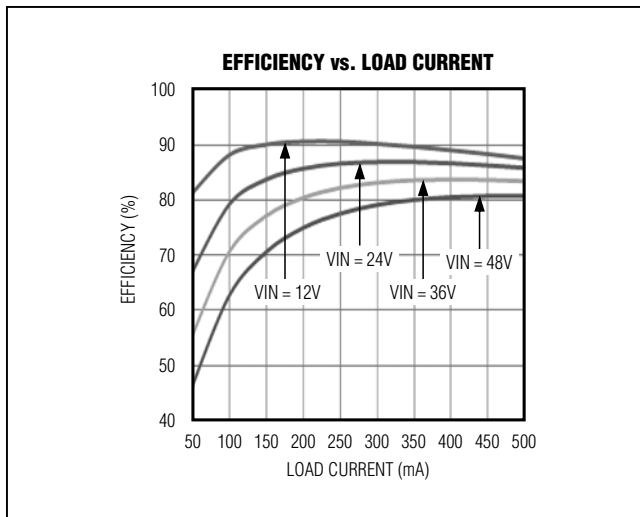
Figure 2. MAX17501H Efficiency
