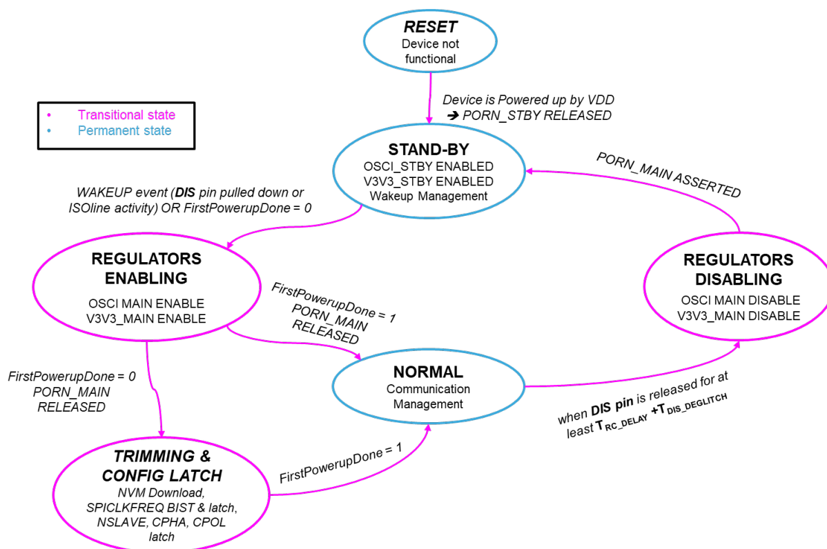
Figure 12. L9963T FSM
