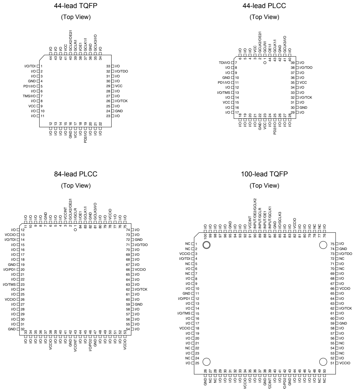
Figure 1-1. Pinouts
