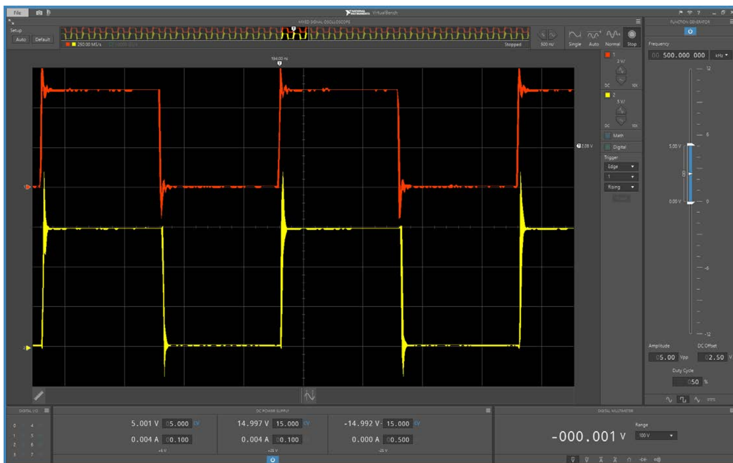
Figure 2.1. 500 kHz Square Wave
