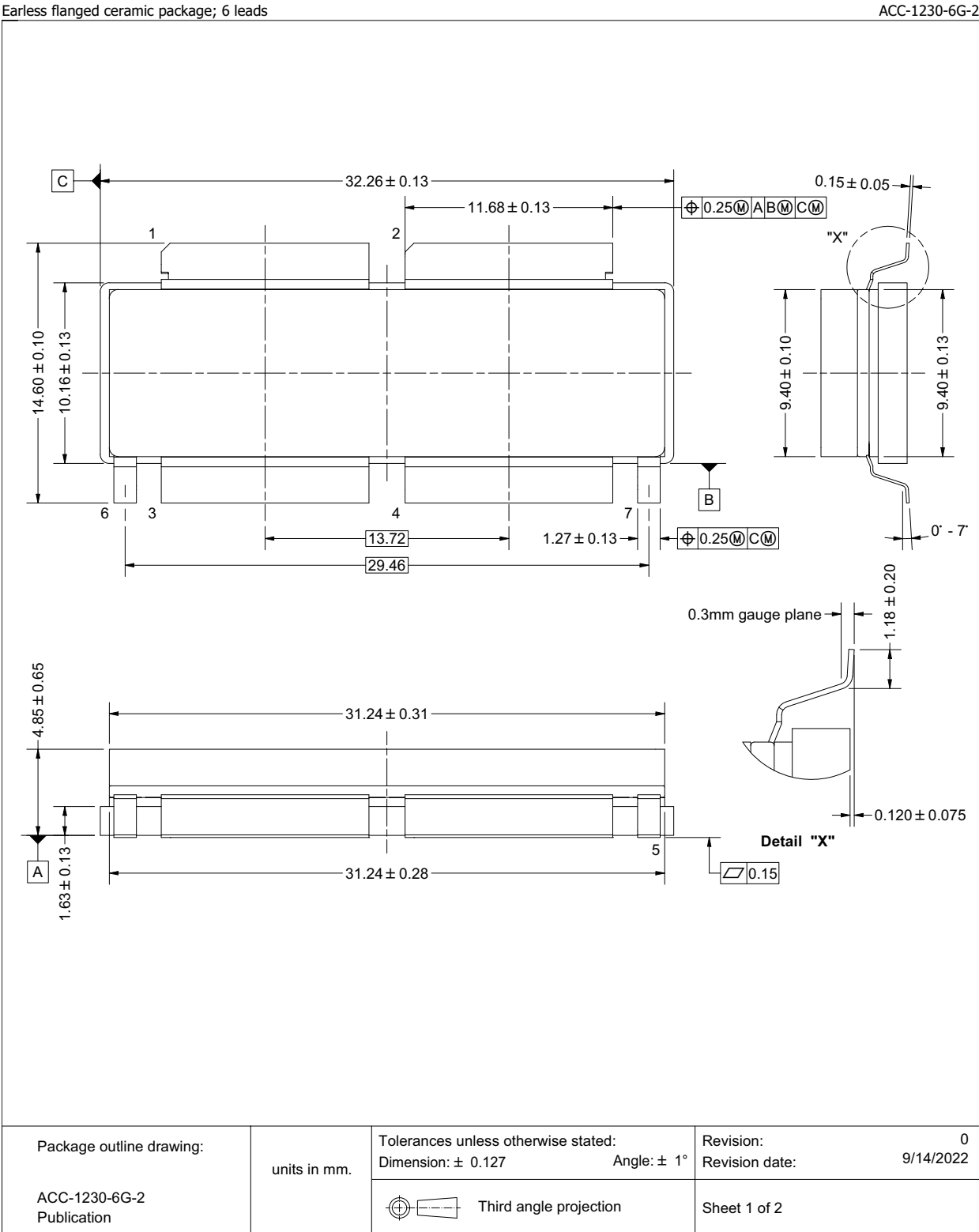
Fig 14. Package outline ACC-1230-6G-2 (sheet 1 of 2)
