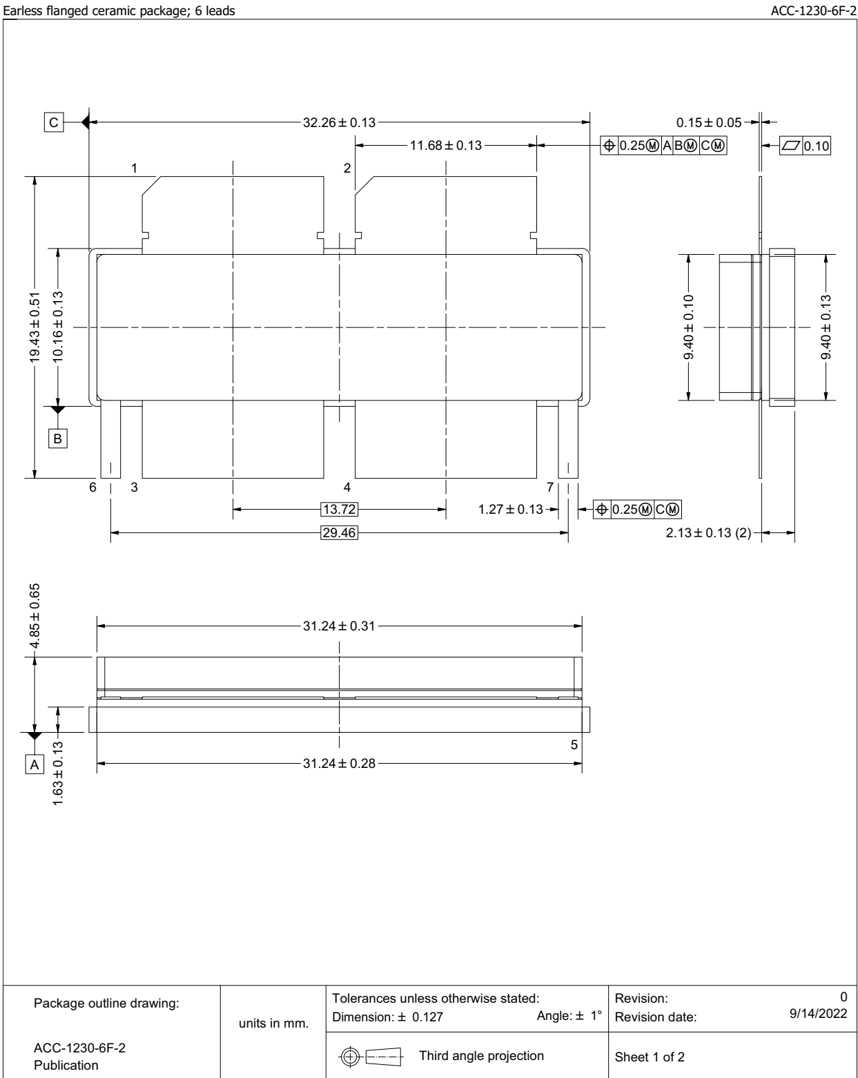
Fig 12. Package outline ACC-1230-6F-2 (sheet 1 of 2)
