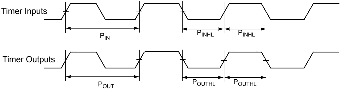
Figure 10-14 Timer Timing
