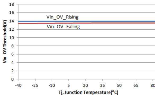
Figure 20. V_{IN\_VOVO} vs. Temperature
