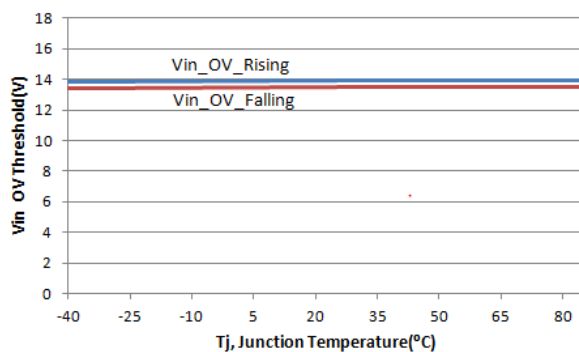
Figure 21. V_{BUS\_VOVO} vs. Temperature
