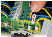
CAGE CLAMP® connection Removing a solid conductor.
