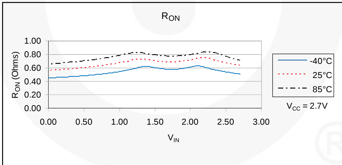
Figure 7. On Resistance
