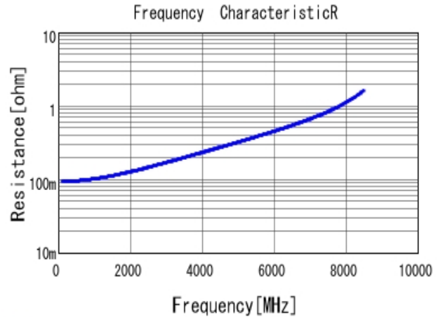
■ GCQ1555C1H6R2DB01 R DC0V, 25degC
