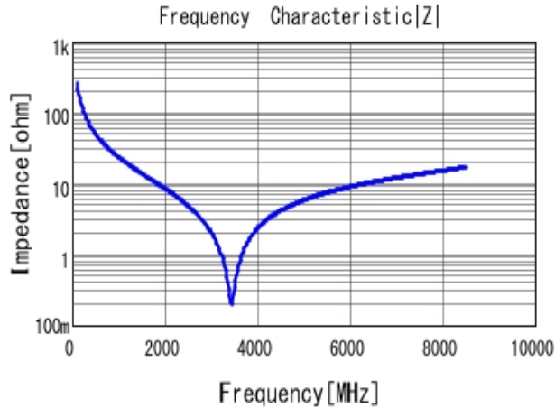
■ GCQ1555C1H6R2DB01 |Z| DC0V, 25degC
