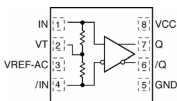
8-Pin DFN
