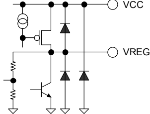
Figure 37. VREG, VCC
