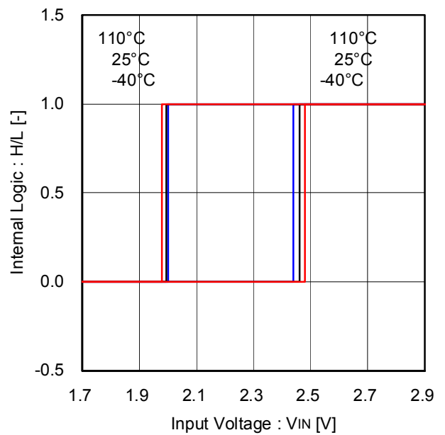
Figure 22. Input threshold voltage (CCW, FIB)
