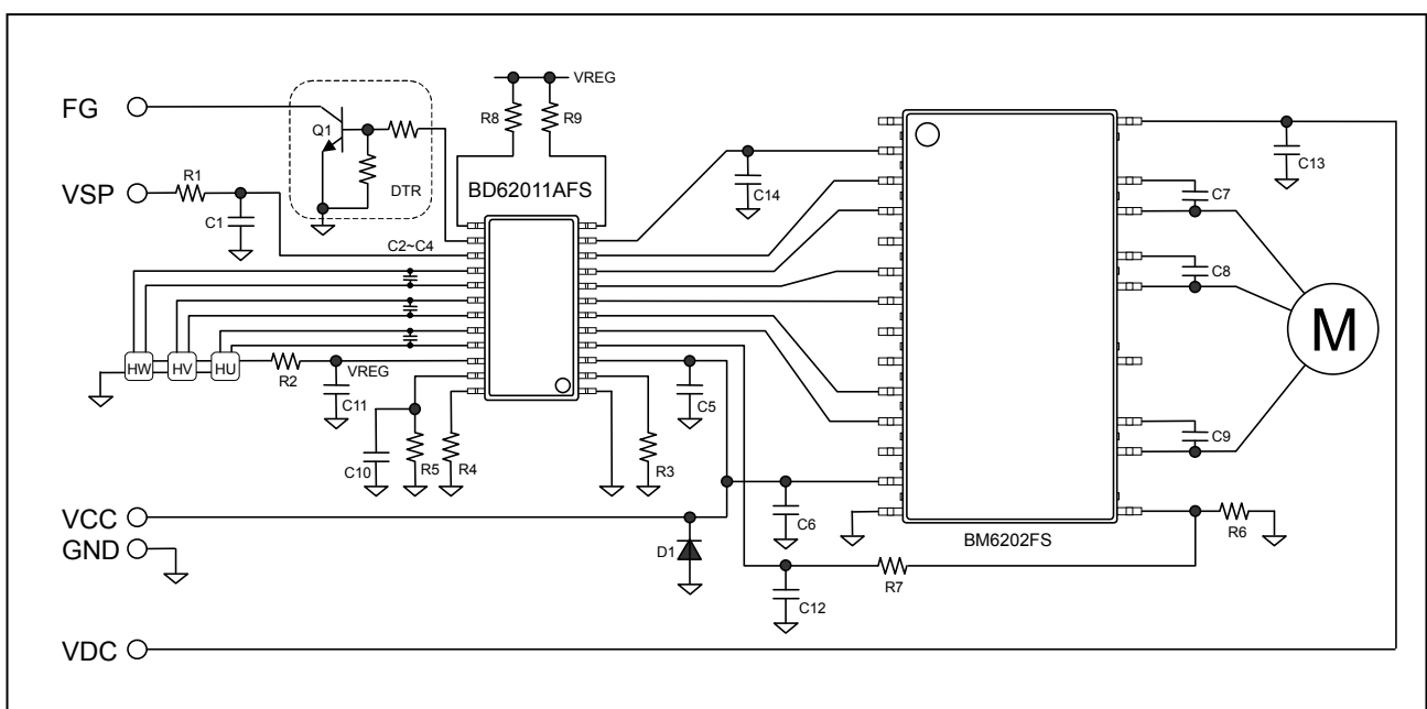
Figure 1. Application circuit example - BD62011AFS &amp; BM6202FS
