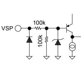
Figure 36. VSP
