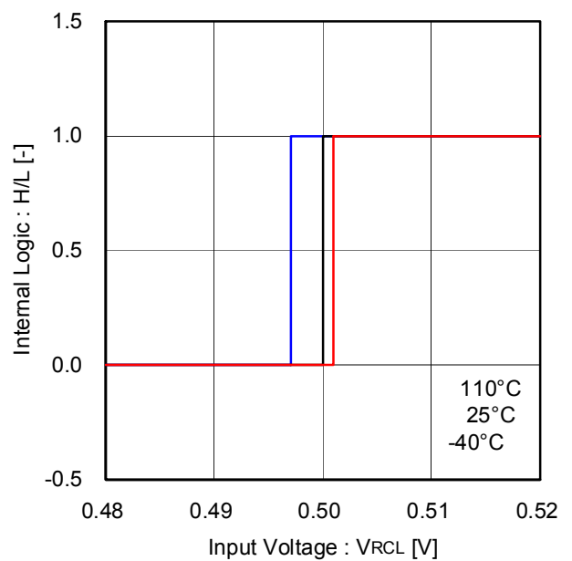
Figure 24. RCL input threshold voltage
