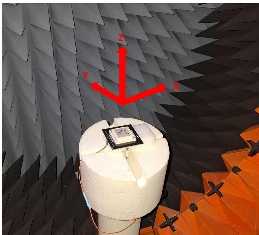
Chamber Test Set-up
