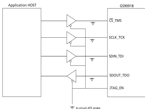
Figure 3-21: In-Circuit JTAG
