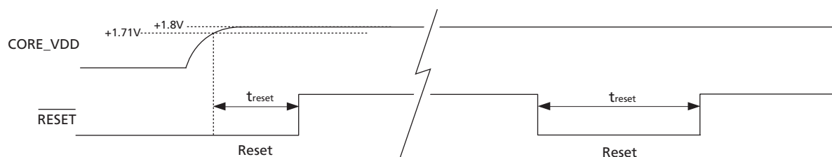
Figure 3-23: Reset pulse
