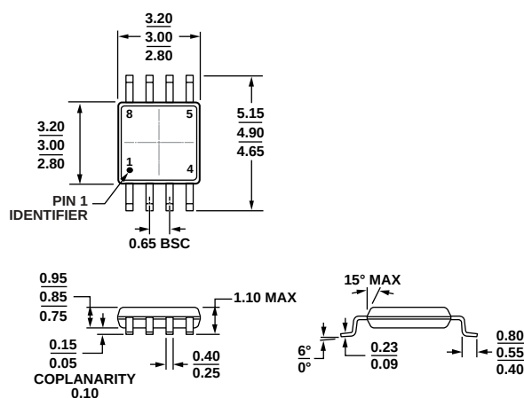
COMPLIANT TO JEDEC STANDARDS MO-187-AA Figure 44. 8-Lead Mini Small Outline Package [MSOP] (RM-8) Dimensions show in millimeters
