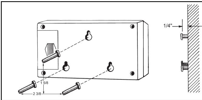
Figure 8. Combo Tester keyhole slots
