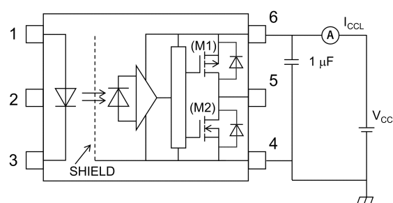
Fig. 13.1.6 I_{CCL} Test Circuit
