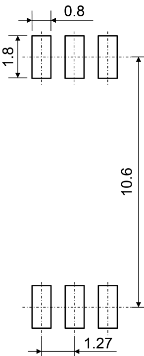
Fig. 15.2 Lead Forming Option (LF4)
