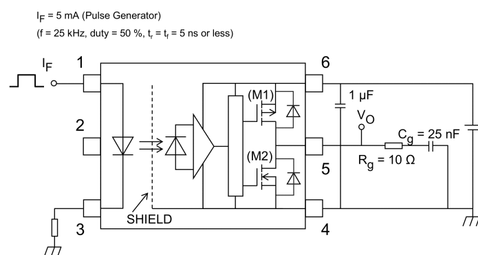
Fig. 13.1.7 Switching Time Test Circuit and Waveform
