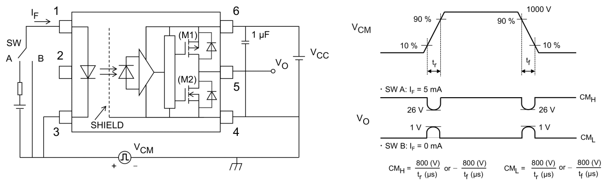
Fig. 13.1.8 Common-Mode Transient Immunity Test Circuit and Waveform
