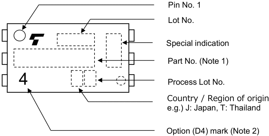
Fig. 17.4 Marking Example
