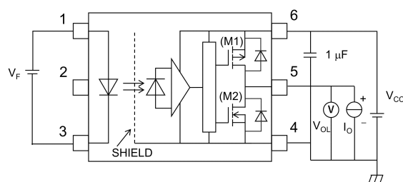
Fig. 13.1.4 V_{OL} Test Circuit
