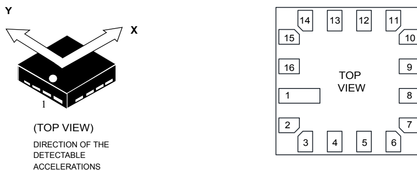
Figure 4. Pin connections
