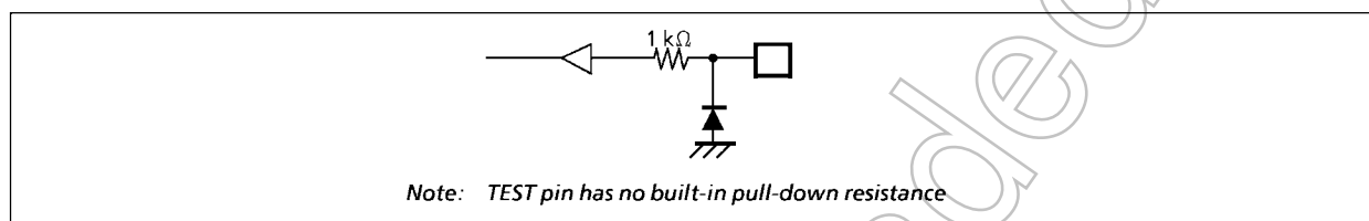
Figure 1-2. TEST Pin
