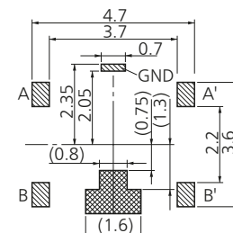
PWB land pattern for reference
