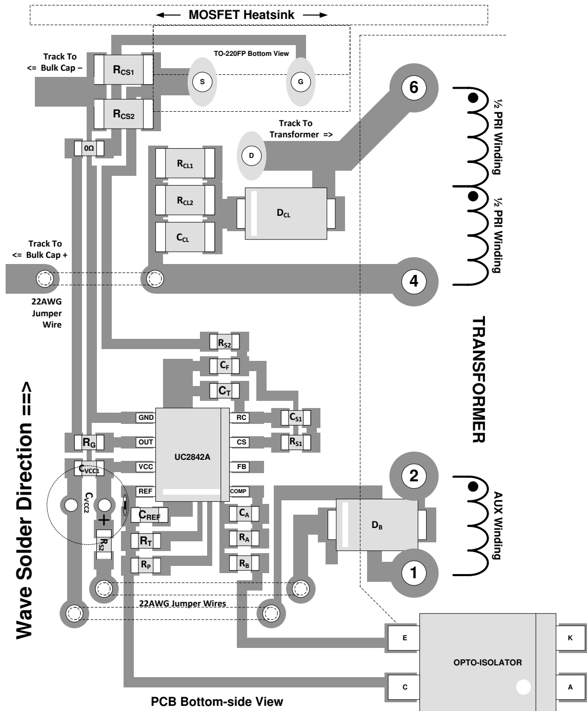
Figure 9-1. Layout Diagram
