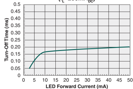
Typical Turn-Off Time vs. LED Forward Current ( I_L=200\text{mA}_{DC} )
