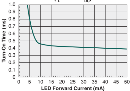
Typical Turn-On Time vs. LED Forward Current ( I_L=200\text{mA}_{DC} )
