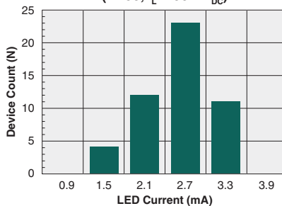
Typical I_F for Switch Dropout (N=50, I_L=200\text{mA}_{DC} )
