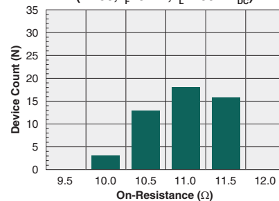
Typical On-Resistance Distribution (N=50, I_F=5\text{mA} , I_L=200\text{mA}_{DC} )
