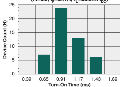
Typical Turn-On Time (N=50, I_F=5\text{mA} , I_L=200\text{mA}_{DC} )
