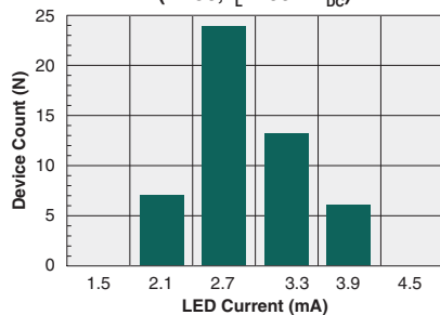
Typical I_F for Switch Operation (N=50, I_L=200\text{mA}_{DC} )
