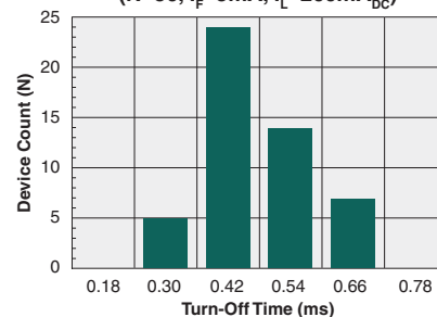
Typical Turn-Off Time (N=50, I_F=5\text{mA} , I_L=200\text{mA}_{DC} )
