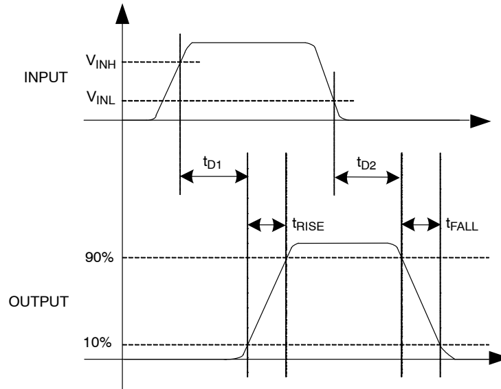
Figure 3. Timing Diagram
