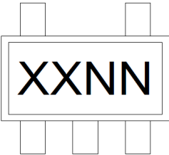
5-Lead SOT-23 (MCP6021/MCP6021R)
