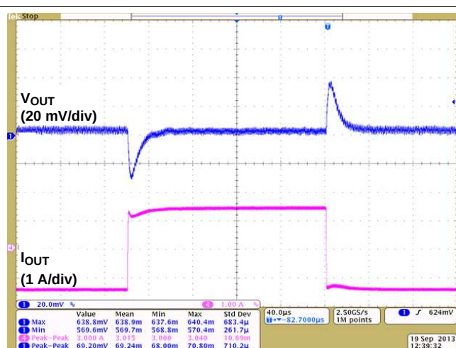
Figure 32. Load Transient
