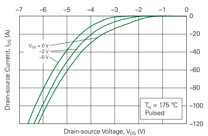
Fig. 12. Body Diode Curves @ T_{vj} = 175\text{ °C}
