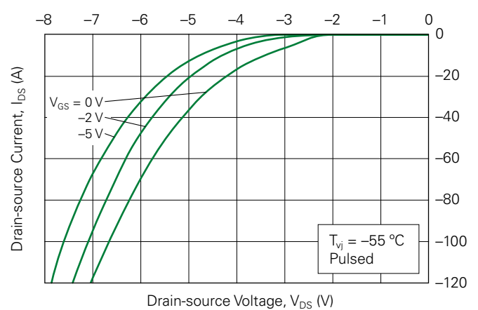
Fig. 10. Body Diode Curves @ T_{vj} = -55\text{ °C}
