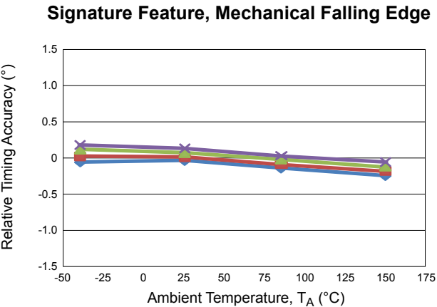
Timing Accuracy versus Ambient Temperature AG = 0.5 mm; relative to T_A = 25^{\circ}\text{C} , S_{\text{ROT}} = 1000\text{ rpm}
