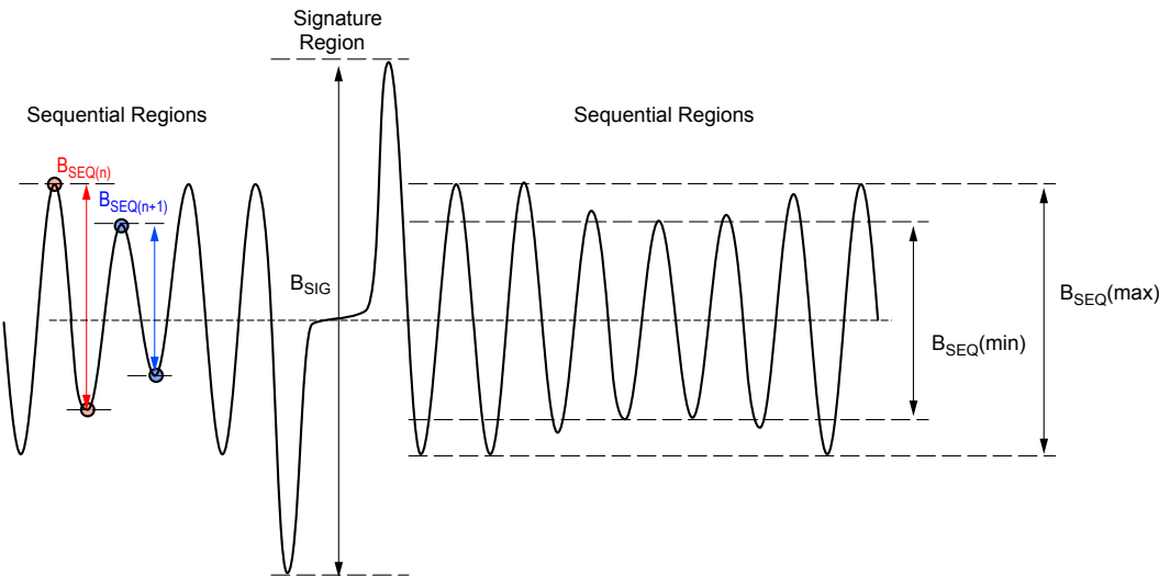
Figure 3. Differential signature amplification and sequential signal variation
