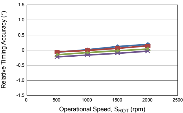
Sequential Features, Mechanical Falling Edge
