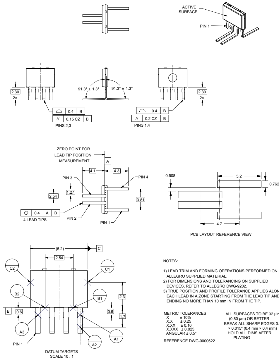
Figure 21: Package KT, 4-Pin SIP, TG Leadform
