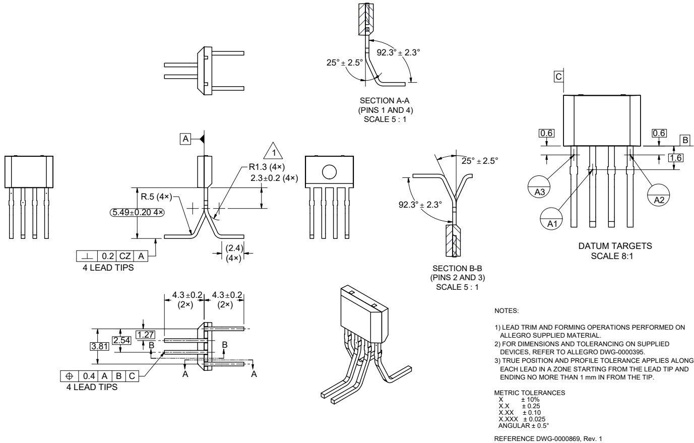
Figure 22: Package OK, 4-Pin SIP, TX Leadform
