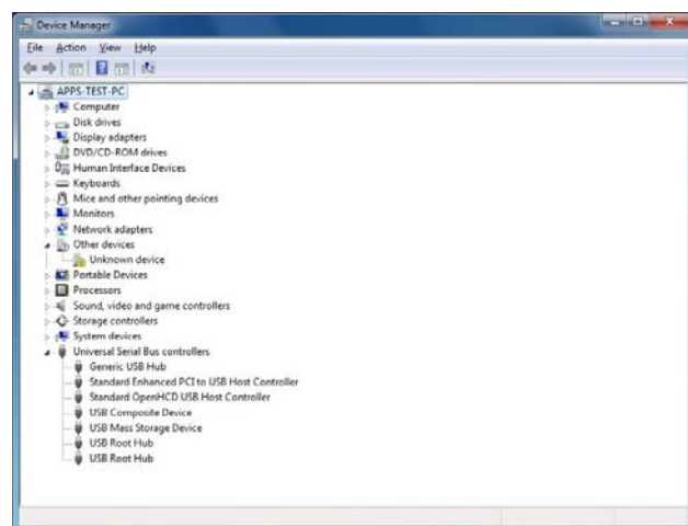
Figure 7. Device Manager
