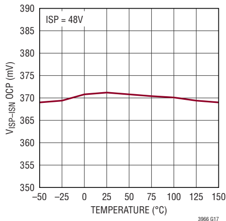
V ISP-ISO Threshold vs Temperature Overcurrent Protection
