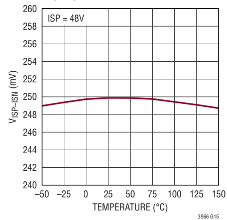
V ISP-ISO vs Temperature
