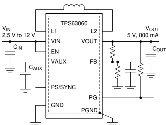
Simplified Application
