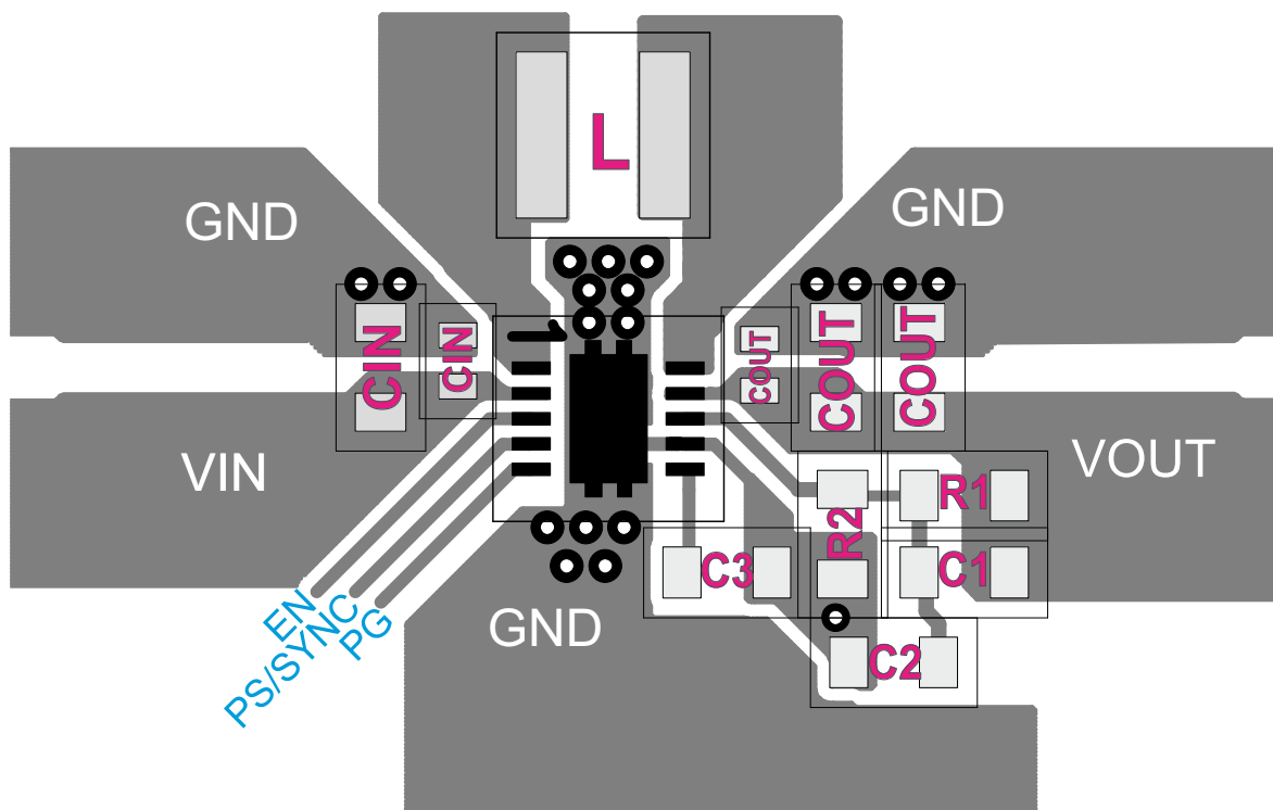
Figure 11-1. TPS6306x Layout
