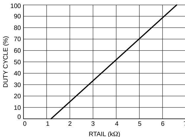
Figure 4. Duty Cycle vs. RTAIL
