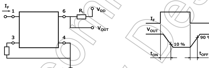
Fig. 12.1 Switching Time Test Circuit and Waveform
