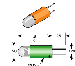
Series: BP203 PN Example: BP200-0AG-014V
