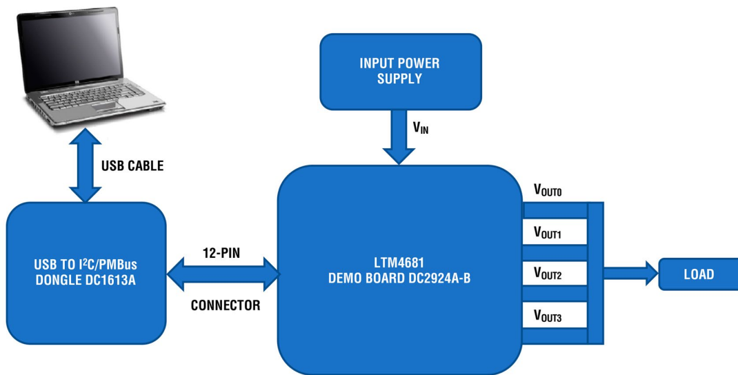
(b) DC2924A-B
