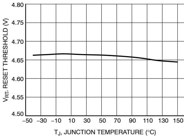
Figure 32. Reset Threshold vs. Temperature (5 V option)
