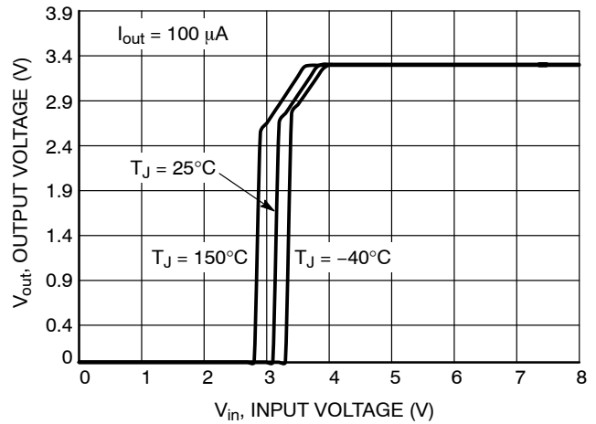
Figure 13. Output Voltage vs. Input Voltage (3.3 V option)
