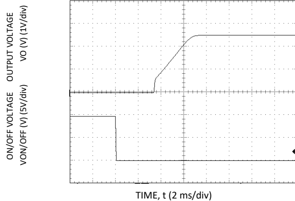
Figure 28. Start-up Using On/Off Voltage ( I_o = I_{o,max} ), V_o = 2.5\text{ V}
