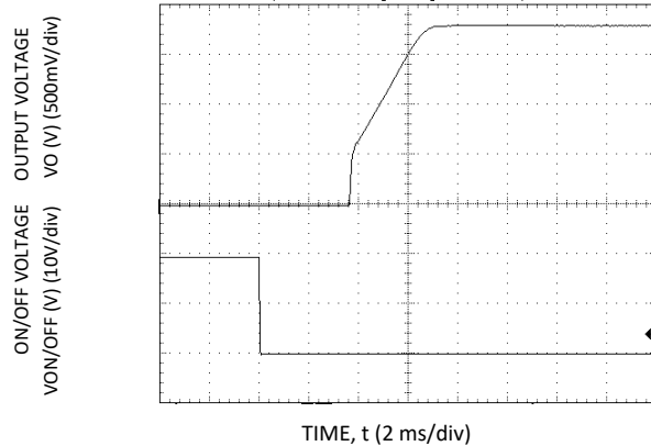
Figure 27. Start-up Using On/Off Voltage ( I_o = I_{o,max} ), V_o = 1.8\text{ V}
